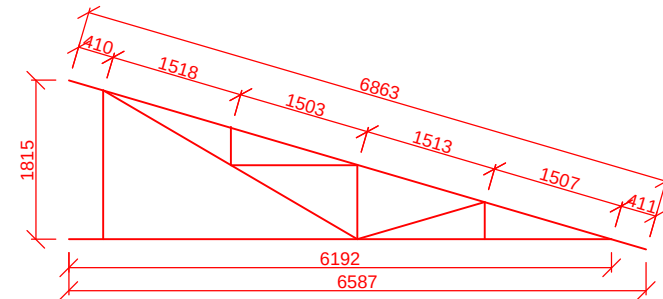
LAYOUT OF TRUSS -A2 (8 NOS.)
