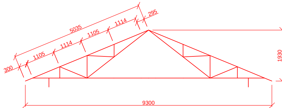
LAYOUT OF TRUSS -A1 (4 NOS.)
