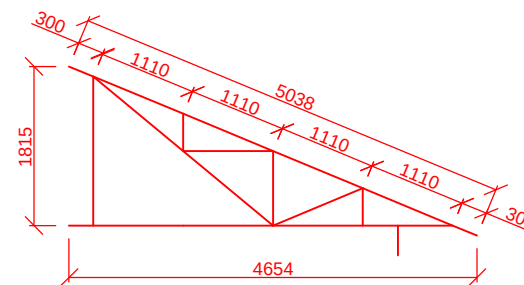
LAYOUT OF TRUSS -A3 (4 NOS.)
